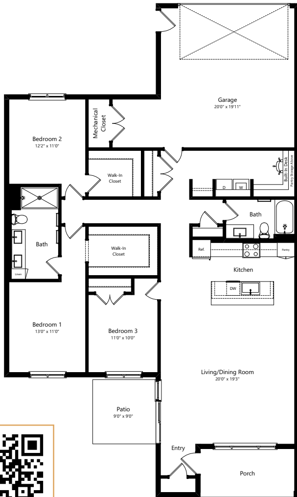
2D PLAN
